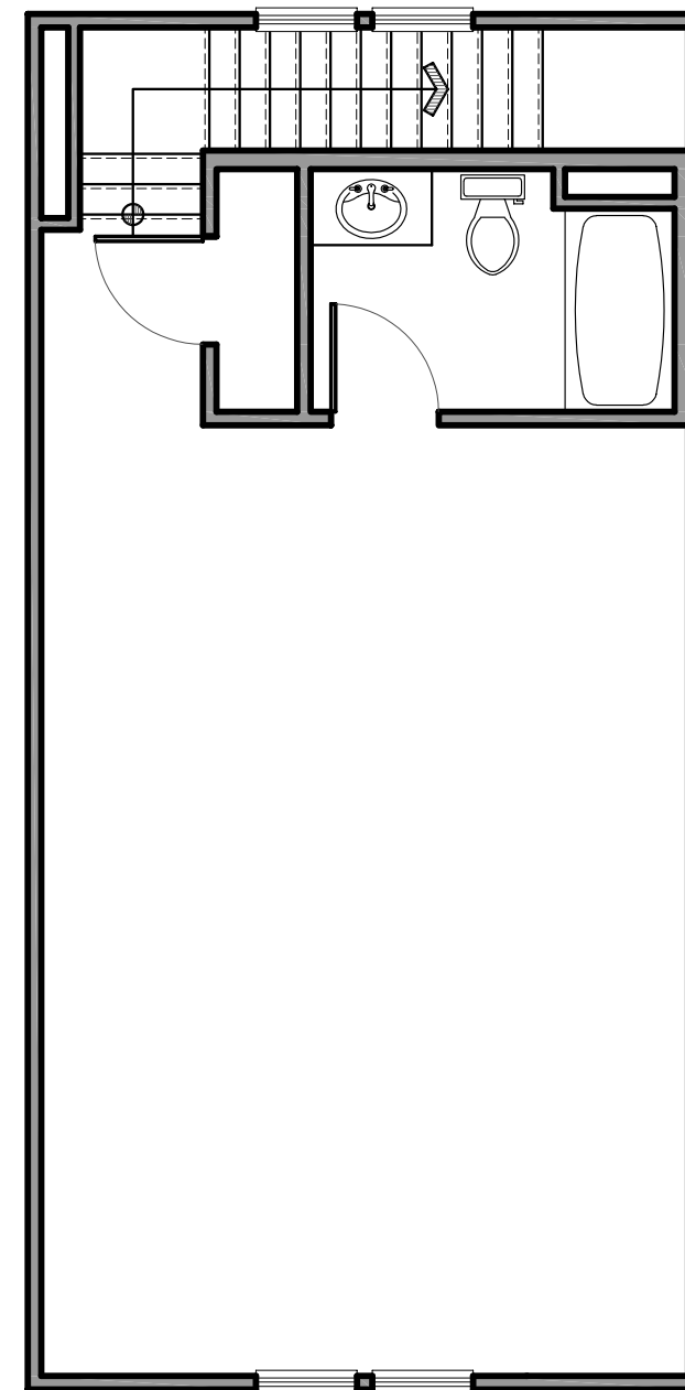
Second Floor
