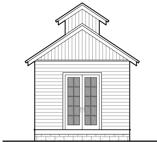
Rear Elevation
