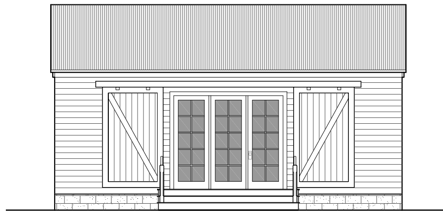
Rear Elevation
