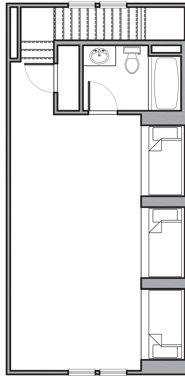
Second Floor
