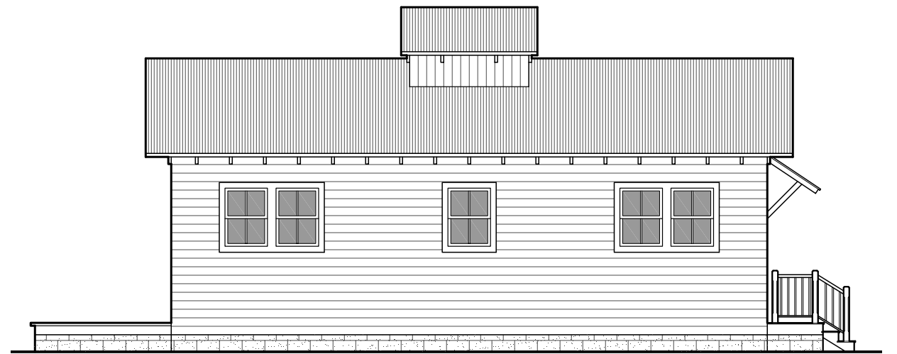
Left Elevation
